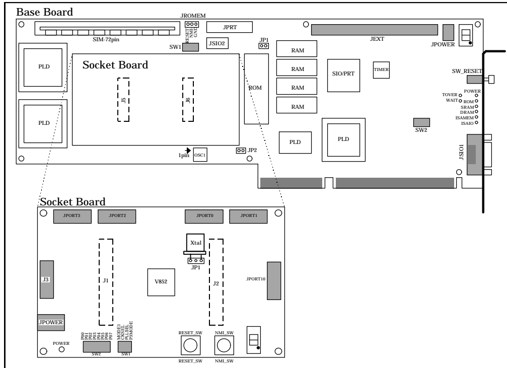
RTE-V852-PC Board Top View
