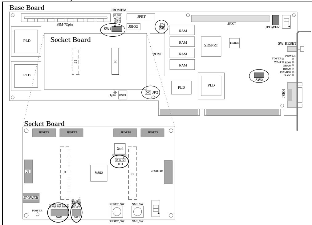
Switches on the RTE-V852-PC Board
