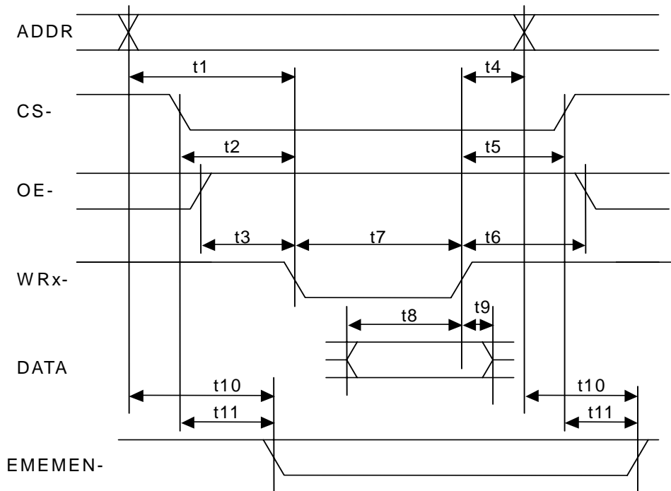
AC Characteristics (1.8V <math>V_{DD} \le 3.3V</math>: V_{DD} = PSENSE(V_{DD IN}) of ROM-IF
